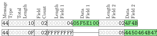
Figure 5: PostgreSQL result set wire format
