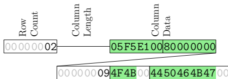
Figure 10: Proposed result set wire format – MonetDB
